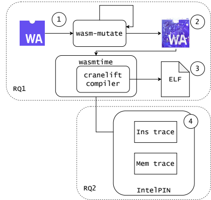
Figure 4: Protocol to answer RQ1 and RQ2
