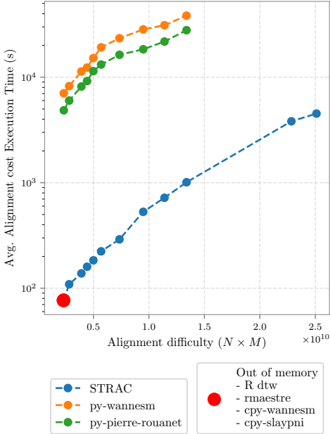
Figure 5. Execution time for 12 trace pair comparisons by 7 tools incl. STRAC. Y axis is in logarithmic scale. Four tools fail even on the smallest traces.
