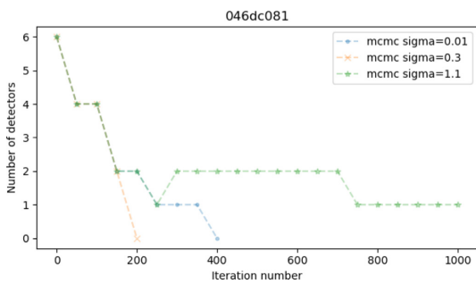
Fig. 4. The figure shows the MCMC evasion process for the binary 046dc081. Each point in the x-axis represents 50 iterations, and the y-axis represents the number of VirusTotal detectors. The figure shows less chaotic progress for oracle evasion.
