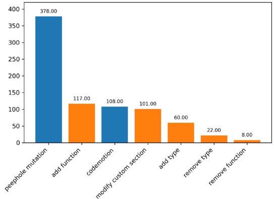
Fig. 6. Distribution of applied transformation for the MCMC evasion algorithm with \sigma = 1.1 (low acceptance). The x-axis displays the names of the transformations. The y-axis indicates the number of transformations found in the generated variants. We can observe which transformations perform better in order to provide total evasion.
